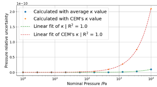
Figure 10. Relative uncertainty of calculated pressure with \kappa obtained by [1] and \kappa calculated by the CEM with Solid Edge software versus the nominal pressure. R^2 is the linear correlation coefficient.
