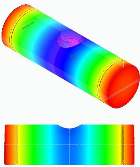
Figure 13. Cylindrical cavity deformation for a pressure of 80 kPa.
