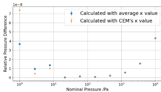
Figure 8. Relative difference between calculated pressure and nominal pressure ( (P_{\text{Nominal}} - P)/P_{\text{Nominal}} ).
