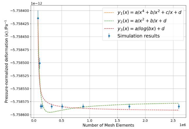
Figure 14. Pressure-normalized deformation versus the number of mesh elements. The data were fitted to three equations.
