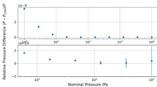
Figure 9. Relative difference between calculated pressure and nominal pressure ( (P - P_{\text{CEM}})/P ), where P is the nominal pressure and P_{\text{CEM}} is the calculated pressure. In the first figure the uncertainty is not appreciable, but in the enlargement below the uncertainty can be seen.
