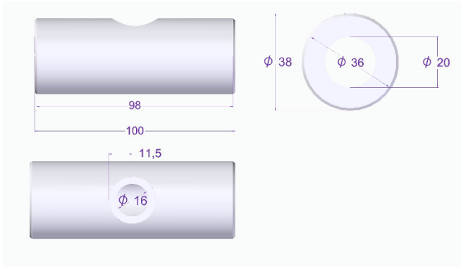
Figure 12. Dimensions of the Zerodur spacer in mm.
