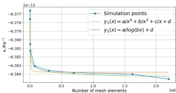
Figure 5. Pressure-normalized deformation versus number of mesh elements. The data was fitted to two curves
