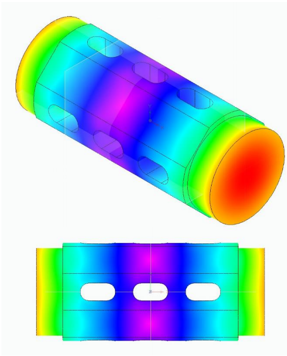
Figure 4. Cavity deformation for a pressure of 80 kPa.
